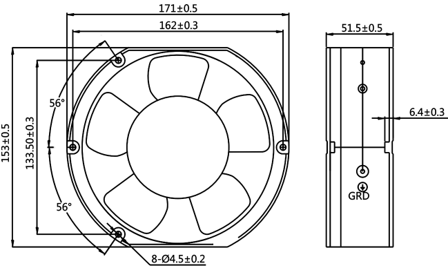
Mechanical Dimensions (mm)
